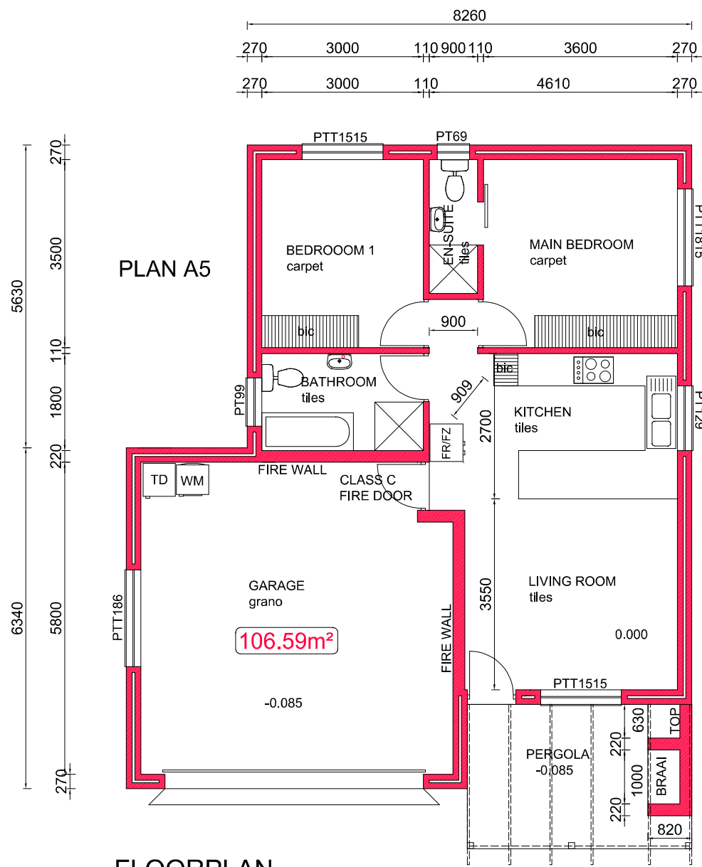
FLOORPLAN SCALE 1:100
