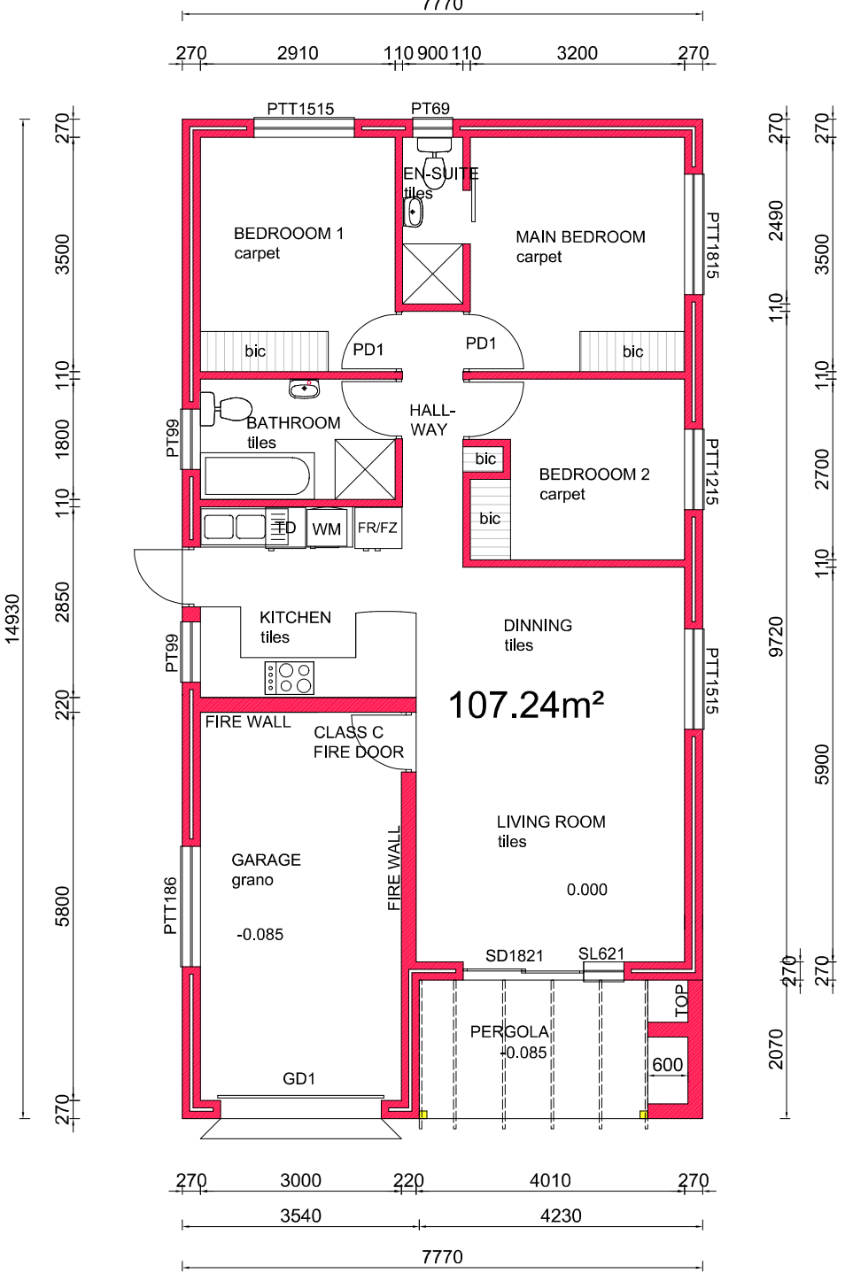
FLOORPLAN SCALE 1:100
